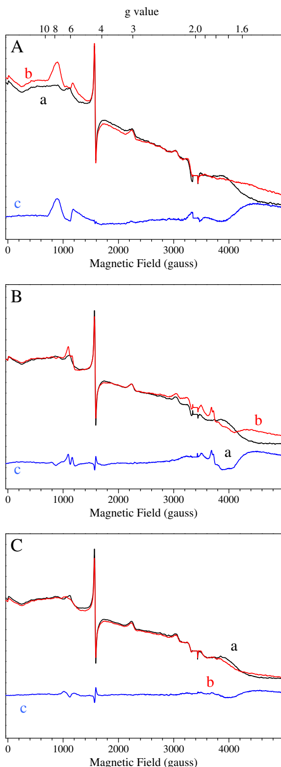
Fig. 1. EPR spectra recorded in PsbA3-PSII at 4.2 K. Effect of the addition of PPBQ (panel A), of DCMU (panel B), and of bromoxynil (panel C). Spectra a (black spectra) were recorded in dark-adapted PSII, spectra b (red spectra) were recorded after the addition of either PPBQ or DCMU or bromoxynil and spectra c (blue spectra) are the difference spectra after minus -before the addition. Other instrument settings: [Chl] = 1.1 mg ml -1 ; modulation amplitude, 25 G; microwave power, 20 mW; microwave frequency, 9.4 GHz; and modulation frequency, 100 kHz. The Tyr D spectral region at g ≈ 2 was deleted.
