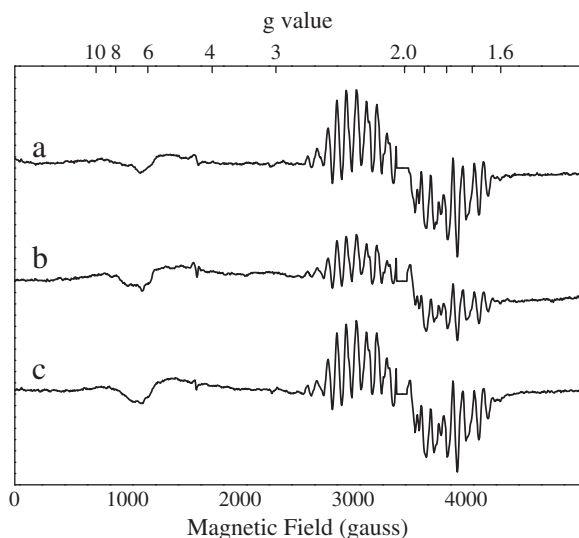
Fig. 9. EPR spectra recorded in PsbA1-PSII at 8.6 K. Spectra were first recorded in dark-adapted samples and then after one flash given at room temperature. The spectra shown are the light-minus-dark spectra in the presence of 3% ethanol (a), of DCMU (b), and of bromoxynil (c). The same other instrument settings as in Fig. 1. The \text{Tyr}_D^{\bullet} spectral region at g \approx 2 was deleted.
