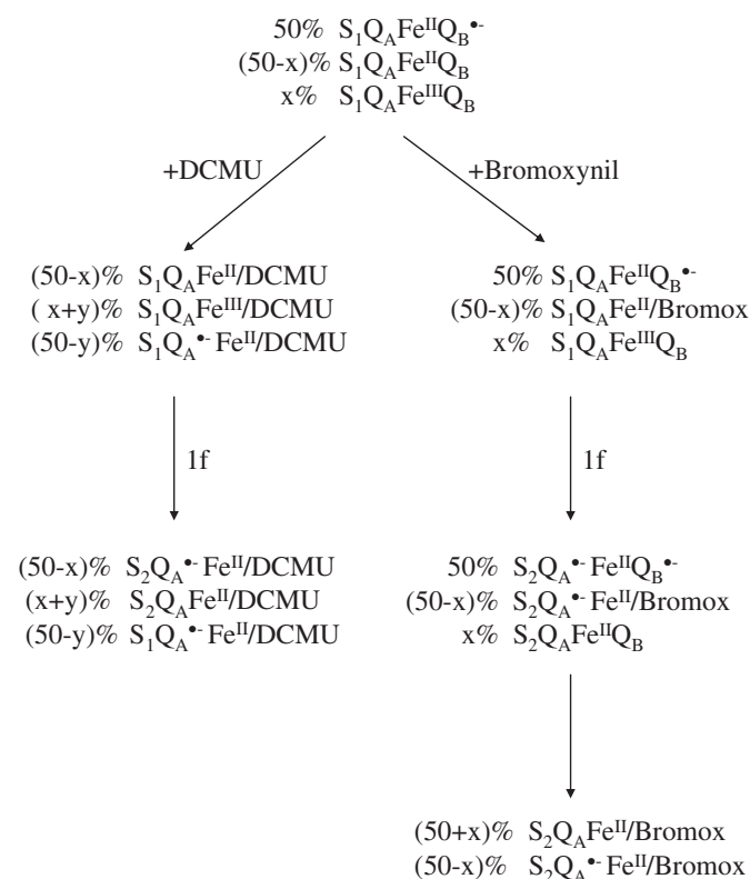
Chart 2. Schematic events following the first flash given on a dark-adapted PSII in the presence of either DCMU or bromoxynil. Centers in the \text{S}_0 state are not considered but they likely behave like those in the \text{S}_1 state.
